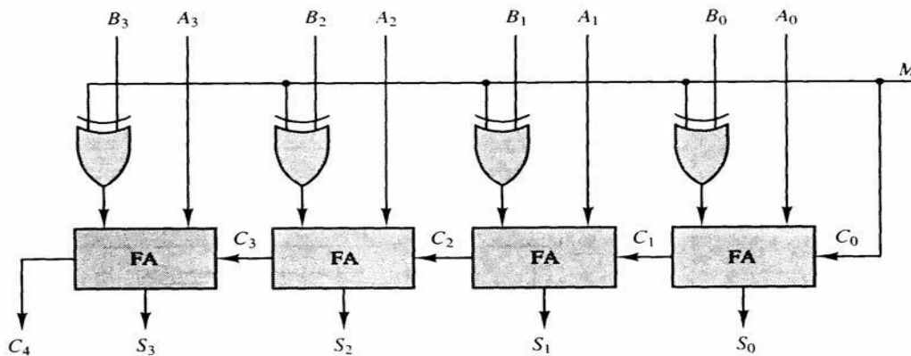
Figure 4-7 4-bit adder-subtractor.
