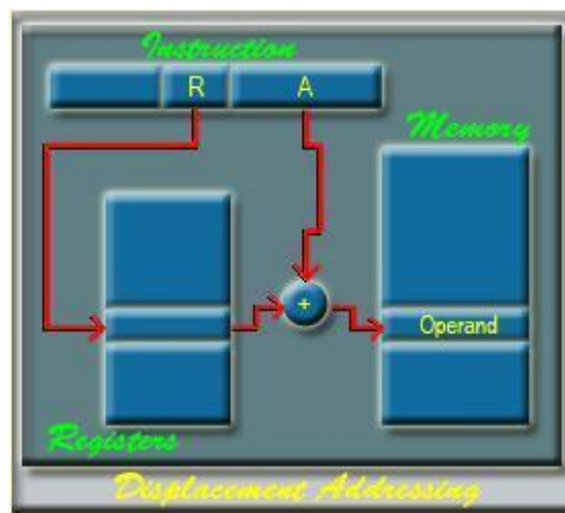
Figure 4.6: Displacement Addressing
